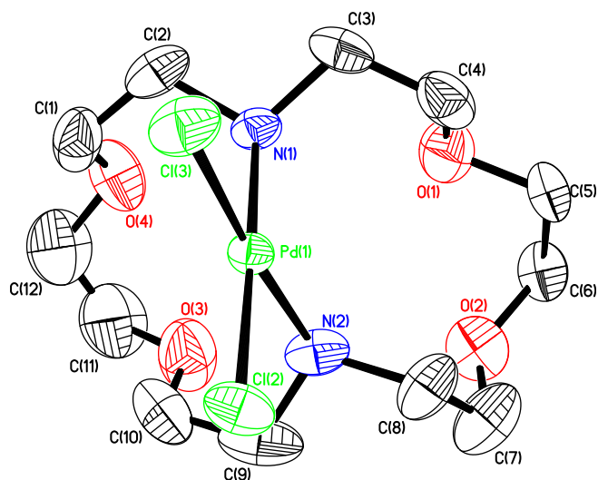
Figure 1. ORTEP drawing of complex 1. Thermal ellipsoids shown at 30% probability level. Hydrogens are omitted for clarity.
